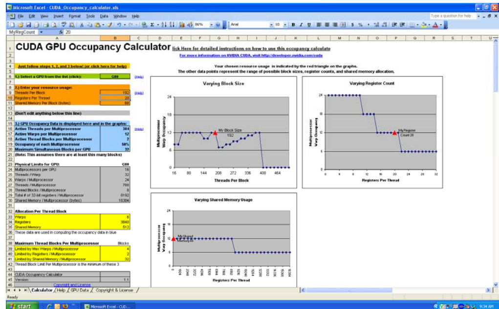
Figure 4.1 Use the CUDA GPU Occupancy Calculator to project occupancy
