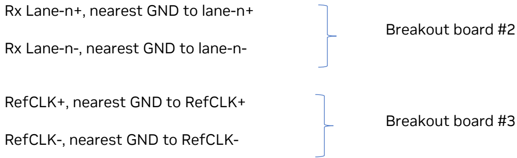
Figure 5. Breakout Board 50 Ω Differential Measurement Use
