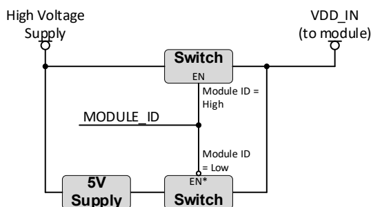
Figure 6-1. System Power and Control Block Diagram
