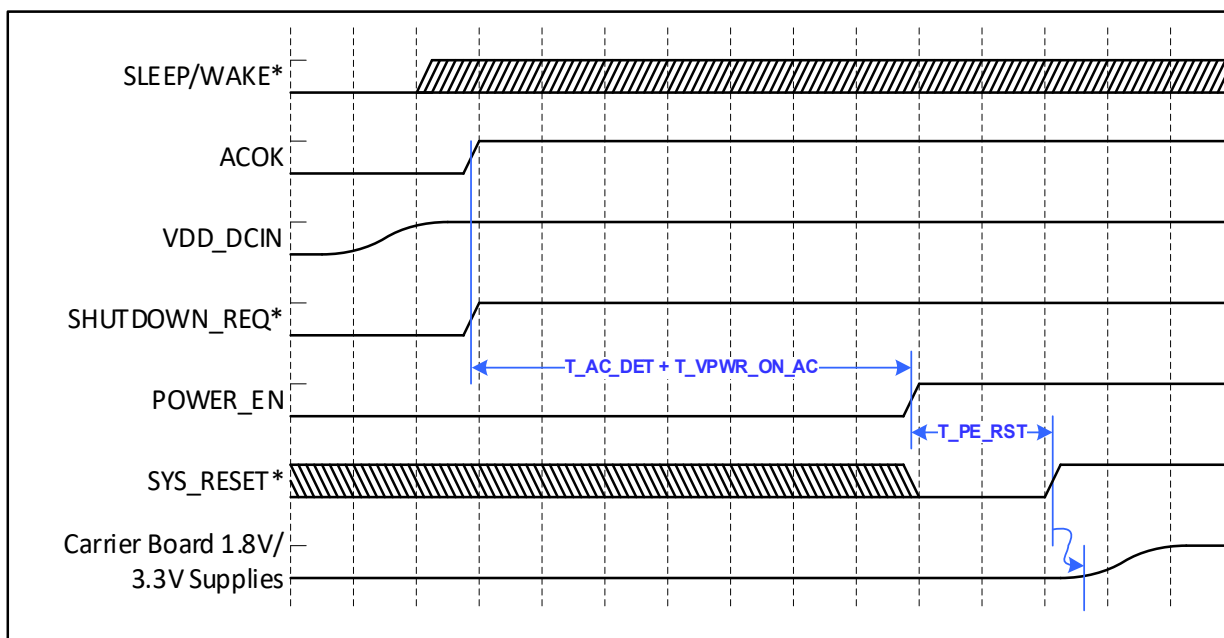
Figure 6-9. Power-Off to On Sequence Auto Power-On Case
