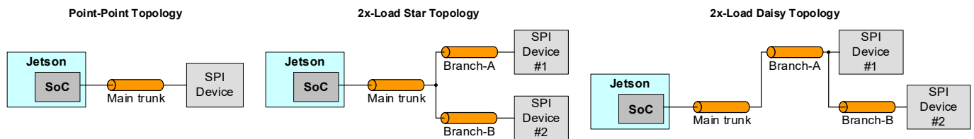
Figure 12-4. SPI Topologies
