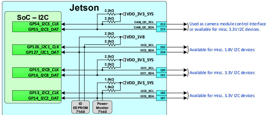
Figure 12-1. I2C Connections
