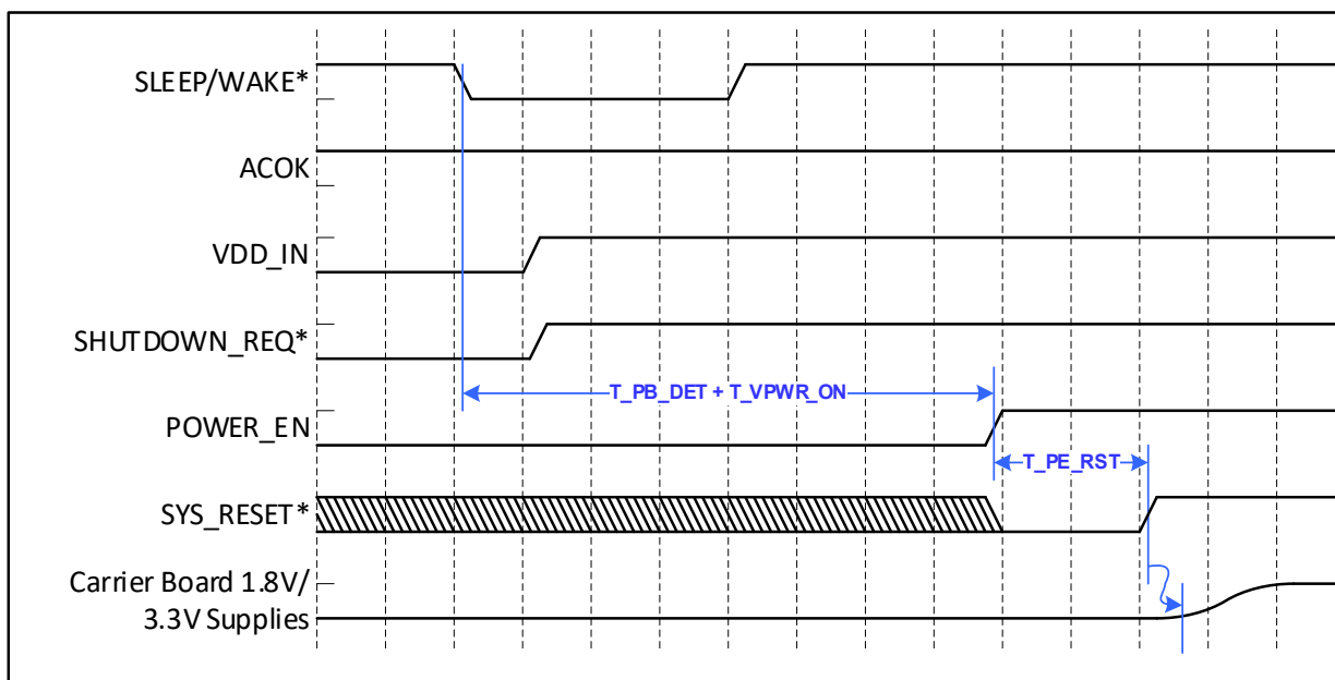
Figure 6-8. Power-Off to On Sequence Power Button Case
