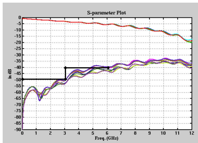
Figure 9-8. IL/FEXT Plot
