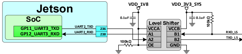
Figure 12-8. Debug UART Connections
