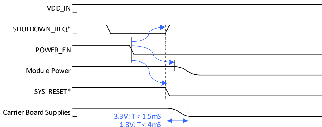
Figure 6-5. Power Down Initiated by SHUTDOWN_REQ* Assertion
