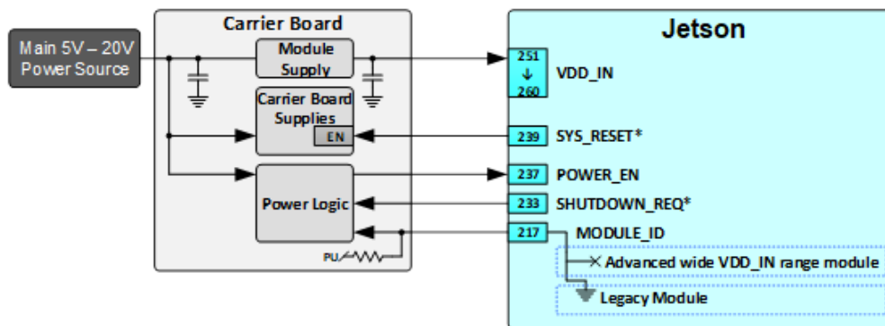
Figure 6-2. System Power and Control Block Diagram
