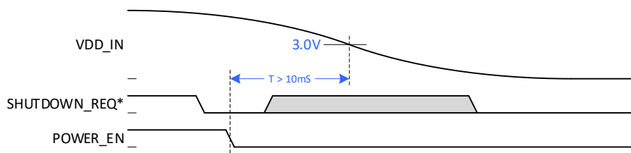
Figure 6-6. Power Down Sudden Power Loss
