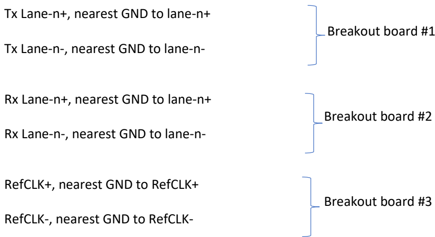
Figure 5. Breakout Board 50 Ω Differential Measurement Use
